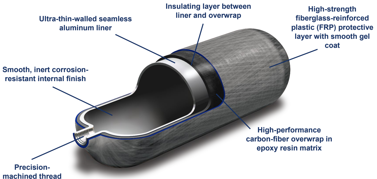
Figure 1: Carbon Composite Cylinder
